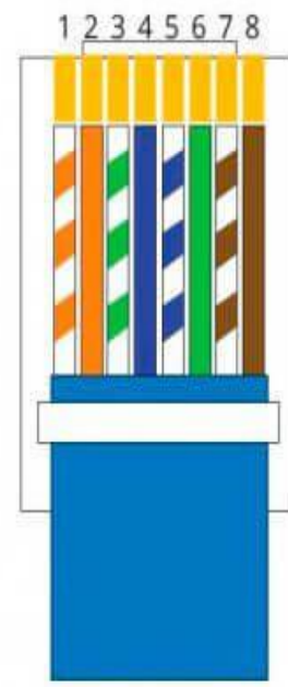
RJ45 Pinout T-568B
