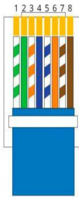
RJ45 Pinout T-568A
